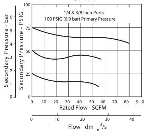
Flow Characteristics 1/4" Port
